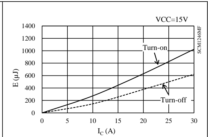
Figure 15-64. Low-side switching loss (T j = 25°C)
