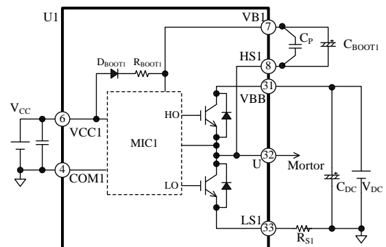
Figure 12-1. Bootstrap circuit
